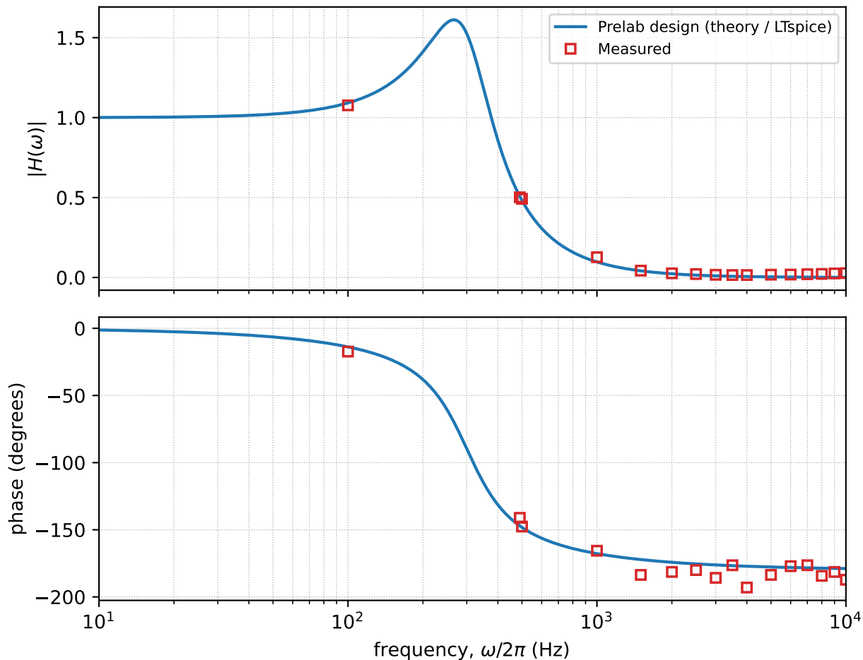
Low-pass Sallen-Key: magnitude and phase response
